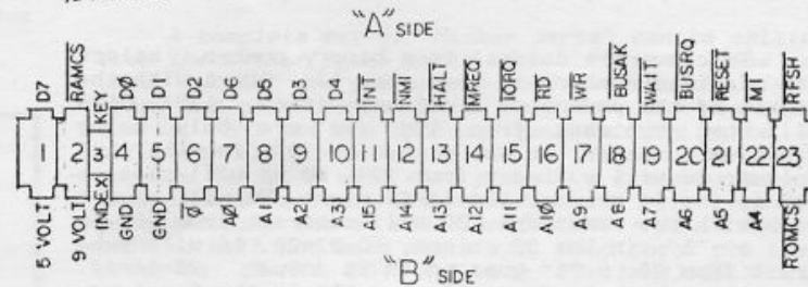
MAIN DECODER COMPONENT DIAGRAM
